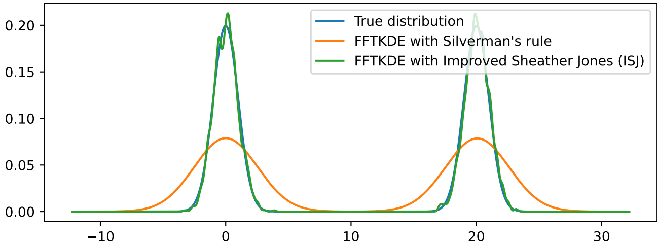
Silverman vs. Improved Sheather Jones
