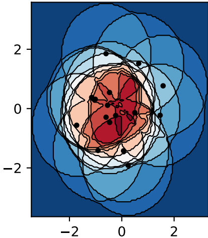
Norm p = 2
