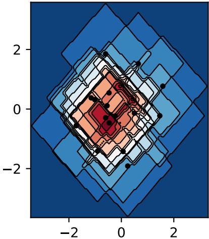
Norm p = 1
