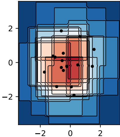
Norm p = \text{inf}
