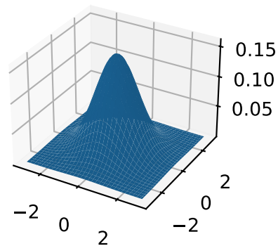
'gaussian', 2-norm
