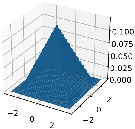
Using the max-norm
