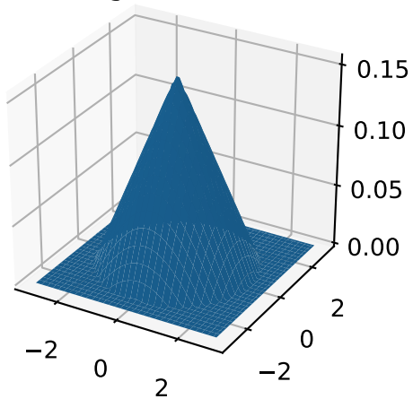
Using the 2-norm
