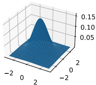
'gaussian', 2-norm
