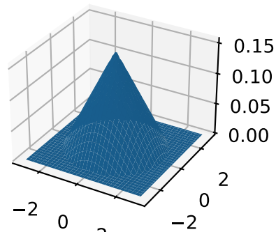
'gaussian', 2-norm
