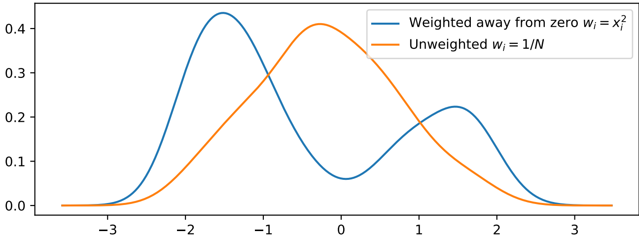
Weighted and unweighted KDE
