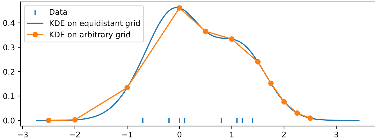
KDE on an equidistant grid by interpolation
